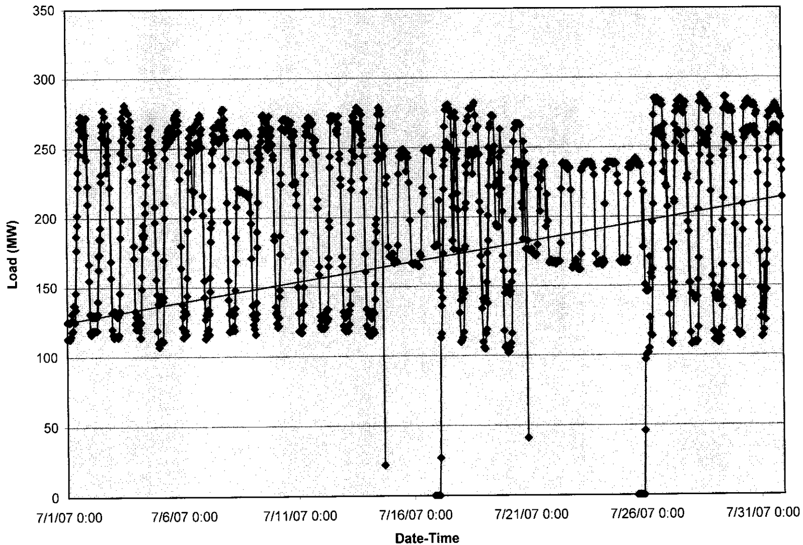
Joliet 71 boiler
